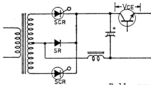
Full-wave rectifier circuit
